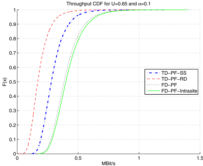
Fig. 2. Throughput CDF for U = 0.65 and \alpha = 0.1
