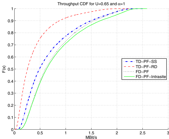
Fig. 3. Throughput CDF for U = 0.65 and \alpha = 1
