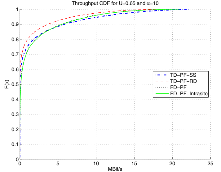
Fig. 4. Throughput CDF for U = 0.65 and \alpha = 10
