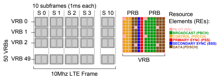
Fig. 1. The essential components of a DL LTE frame.
